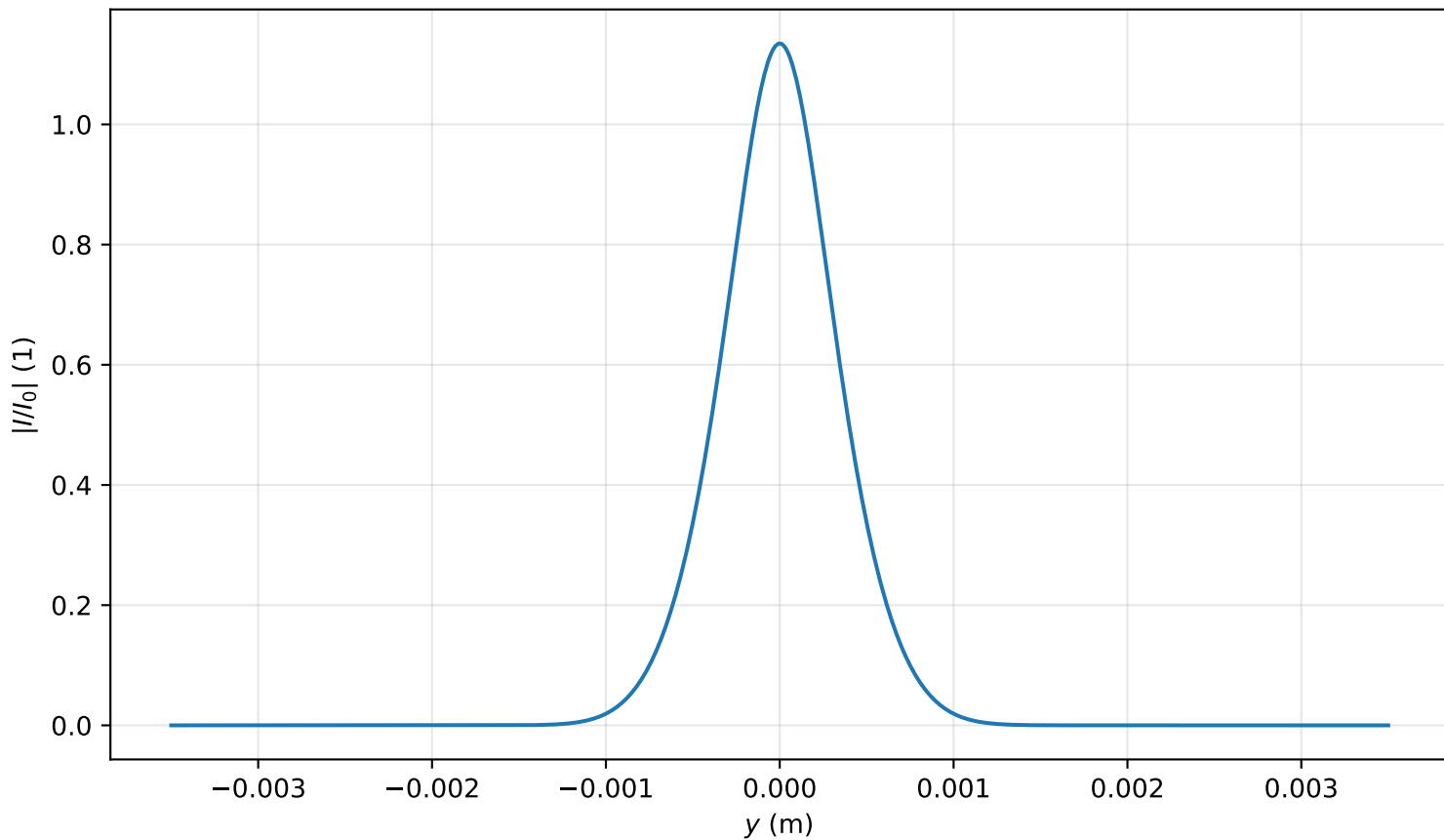
Intensity profile I(x=0, y, z=0.478)/I_0 , \text{Pin}=0.9\text{Pcr} , artificial time
